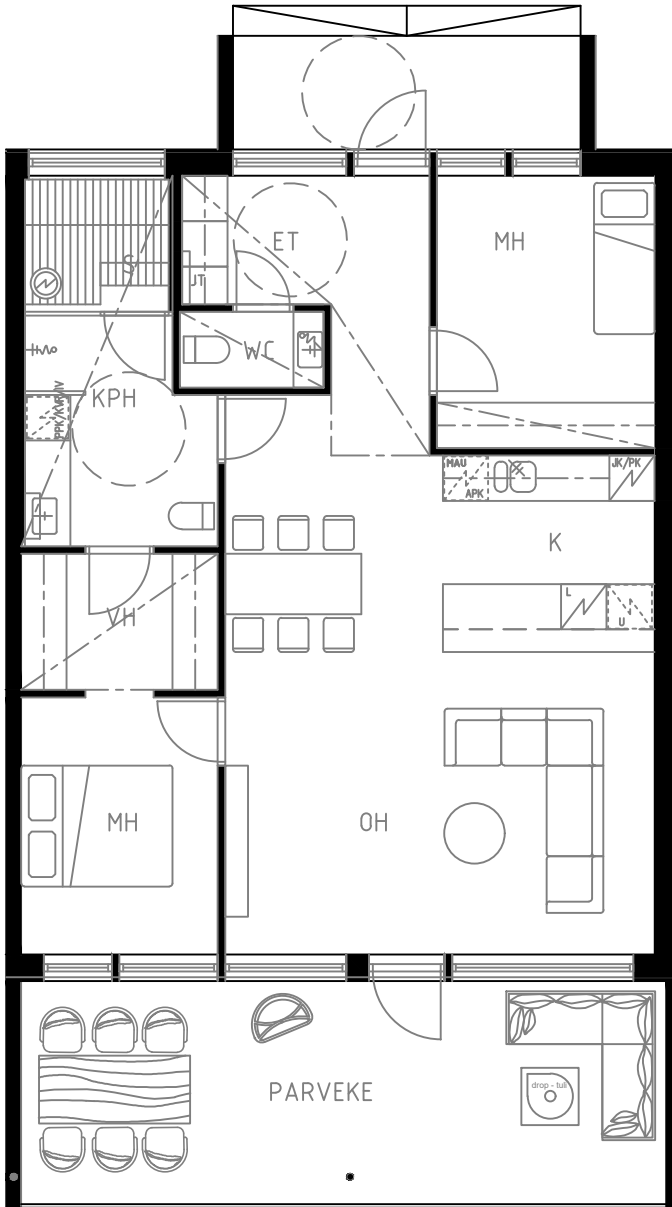
AS A3 3h+k+s 86 m2
